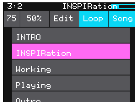
Song Sections
