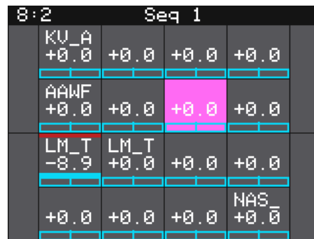
Mixer
