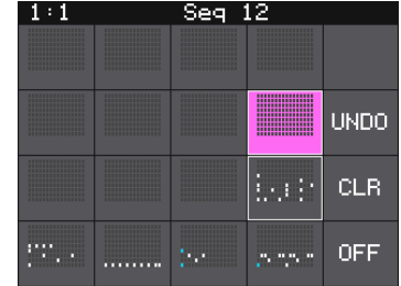
Sequences Grid
